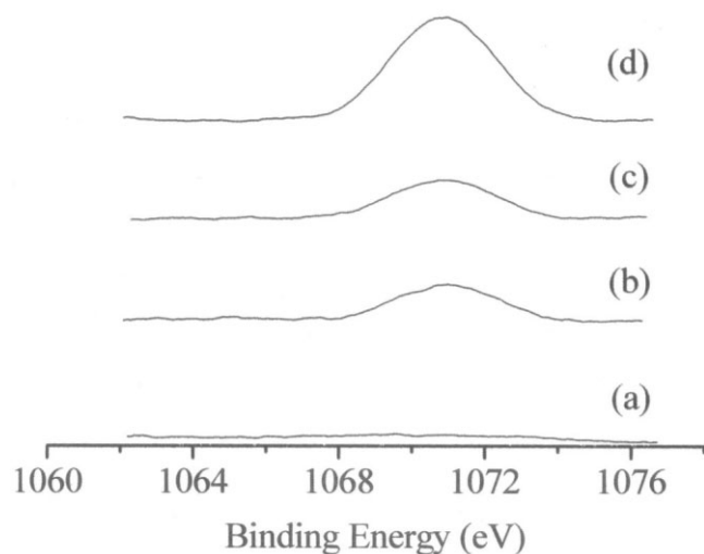
Figure 7 Occurrence of Na by ESCA for membranes treated at 30°C with 1N NaOH at (a) 0.5 h, (b) 2.5 h, (c) 5 h, and (d) 45°C for 5 h.
