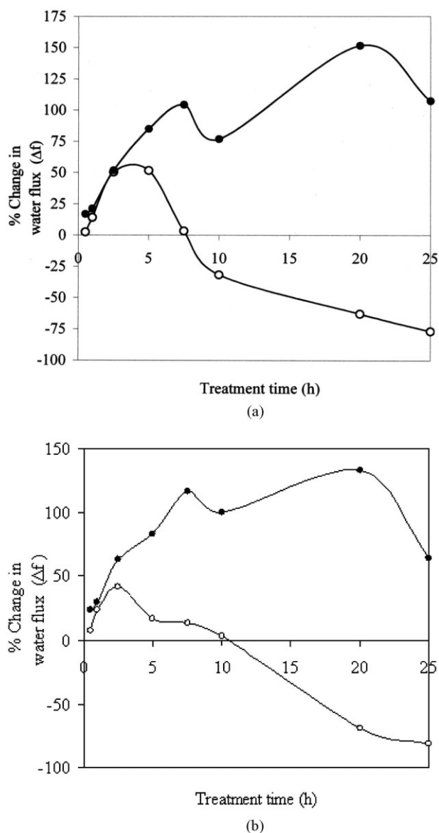
Figure 2 Variation in water flux ( \Delta f ) caused by treatment with dead-end mode in comparison to the untreated membrane; (○) 1N NaOH treatment, (●) 1N NaOH followed by 0.1N HCl treatment.
