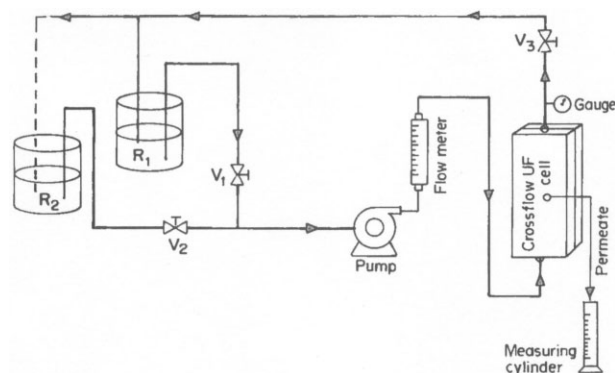
Figure 1 Schematics of crossflow set up.
