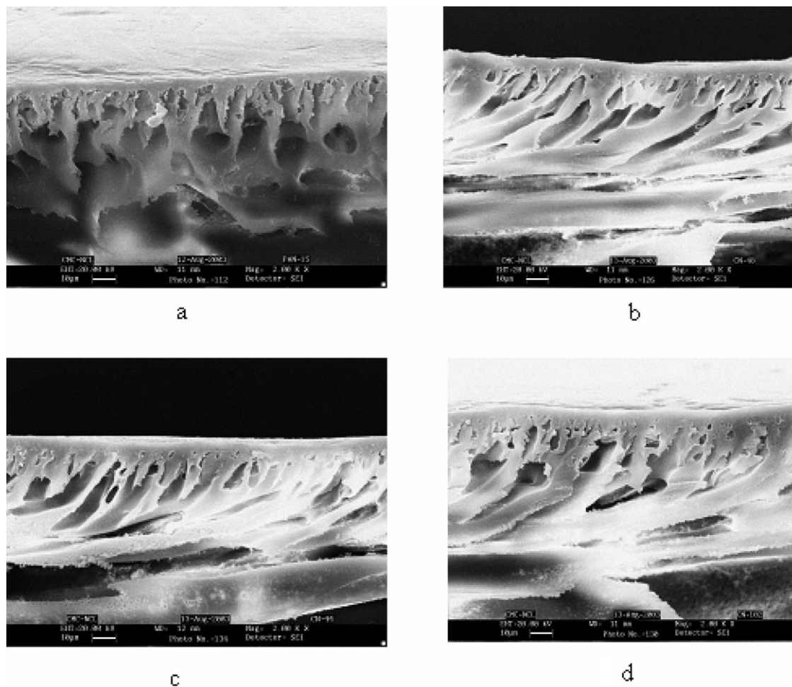
Figure 5 SEM of cross section of PAN membranes; (a) unmodified, (b) 1N NaOH treatment at 30°C for 5 h, (c) 1N NaOH treatment at 30°C for 5 h, followed by 0.1N HCl, (d) 1N NaOH treatment at 45°C for 5 h, followed by 0.1N HCl.
