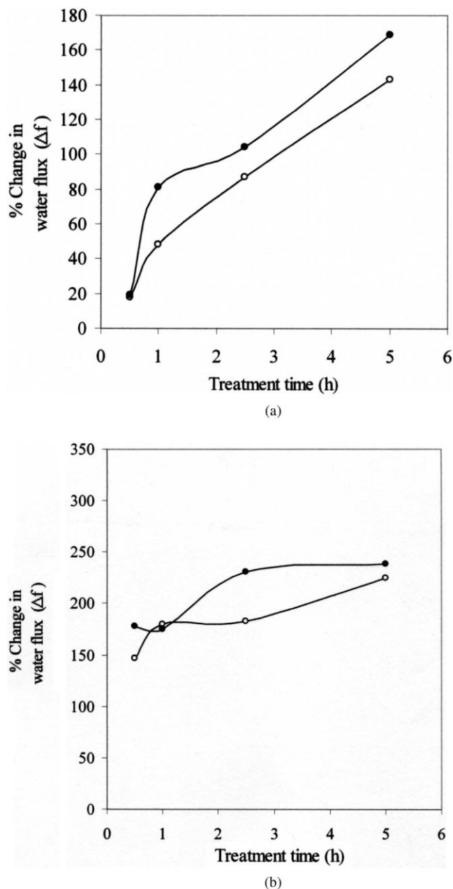
Figure 4 Variation in water flux ( \Delta f ) caused by treatment at 30°C by crossflow mode in comparison to that of untreated membrane; (○) 1N NaOH treatment, (●) 1N NaOH followed by 0.1N HCl treatment.
