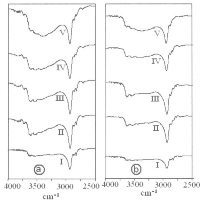
Figure 6 FTIR spectra of PAN powder treated at 45°C with (a) 2.5N NaOH solution, (b) 2.5N NaOH, followed by 0.1N HCl; I: unmodified, II: 0.5 h, III: 1 h, IV: 2.5 h, V: 5 h.
