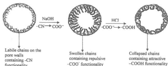
Figure 3 Schematic representation of pore swelling by NaOH treatment and regain of pore size by HCl treatment.
